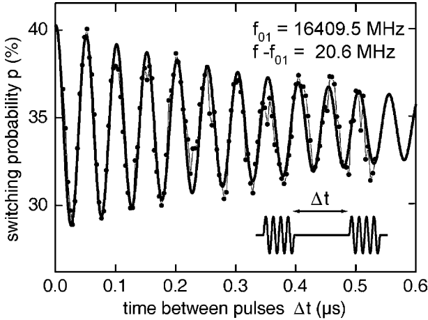
Fig. 13. Measurement of Ramsey fringes for the Quantonium. Two \pi/2 pulses separated by a variable delay are applied to the qubit before measurement. The frequency of the pulse is slightly detuned from the transition frequency to provide a stroboscopic measurement of the Larmor precession of the qubit.
