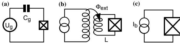
Fig. 4. The three basic superconducting qubits. (a) Cooper pair box (prototypical charge qubit); (b) RF-SQUID (prototypical flux qubit); and (c) current-biased junction (prototypical phase qubit). The charge qubit and the flux qubit requires small junctions fabricated with e-beam lithography while the phase qubit can be fabricated with conventional optical lithography.
