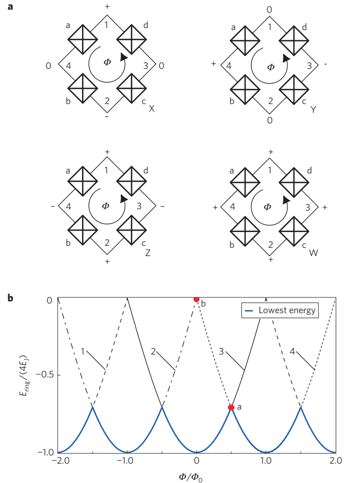
Figure 1 | Electrical modes and energy states of the Josephson ring modulator. a , The Josephson ring modulator consists of four nominally identical Josephson junctions (a, b, c and d) and has four orthogonal electrical modes. The two differential modes X, Y and the common mode Z are coupled to the junctions, whereas the fourth mode W remains uncoupled. b , Energy states of the ring modulator. There are four stable states satisfying the relation \delta_a + \delta_b + \delta_c + \delta_d \bmod 2\pi = 2\pi\Phi/\Phi_0 , where \delta_i is the gauge-invariant phase of junction i and where \Phi_0 is the flux quantum. Each state is 4\Phi_0 periodic as a function of the flux \Phi through the loop, but the envelope (blue line) of the lowest energy remains \Phi_0 -periodic. Other energy extremum states are not represented here. At point a, the device can produce a pure nonlinear coupling term \Phi_X \Phi_Y \Phi_Z , whose contamination is only of the type \Phi_X^2 + \Phi_Y^2 + \Phi_Z^2 . Point a actually corresponds to two degenerate states separated by an energy barrier whose height is 2(\sqrt{2}-1)E_j . At point b, there is no contamination and the nonlinearity is of the purest form, but it would be very difficult to stabilize the device in an excited state.
